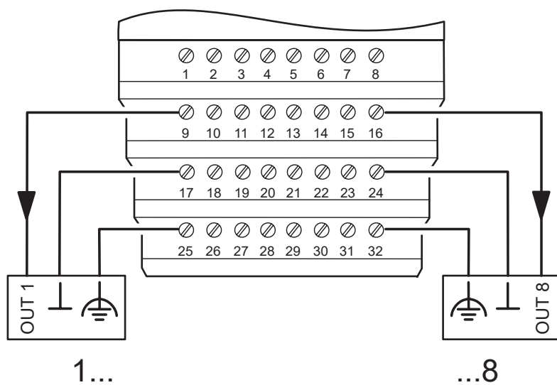
Connection diagram
