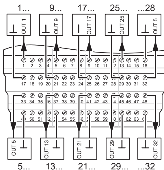
Connection diagram
