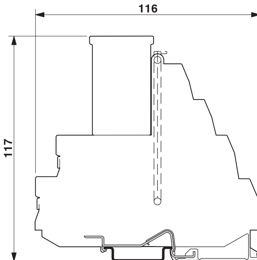
Dimensional drawing
