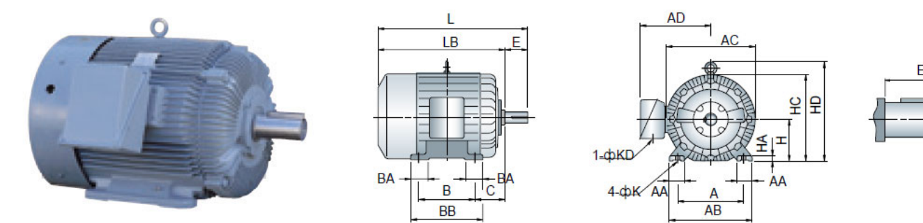
75KW / 100HP 4-pole 50Hz TEFC Induction Motor, Foot Mounted
